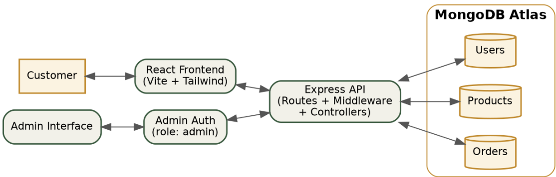
Figure 1: High-level MERN stack architecture flow for the ShopEZ platform
